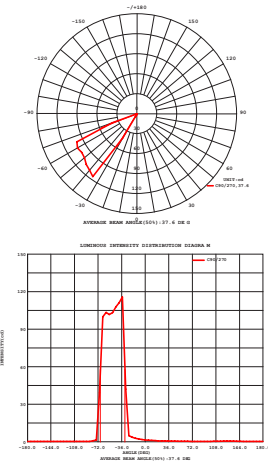
LUMINOUS INTENSITY DISTRIBUTION DIAGRAM
