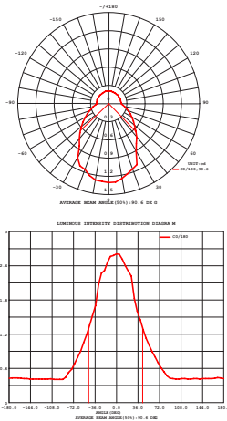
LUMINOUS INTENSITY DISTRIBUTION DIAGRAM
