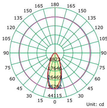
Average Diffuse Angle(50%): 42.0°
