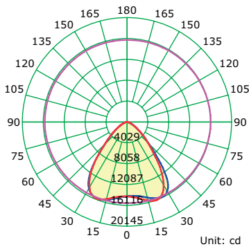
Average Diffuse Angle(50%): 82.8°
